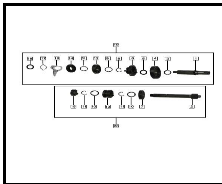
E-18 ARRANQUE
