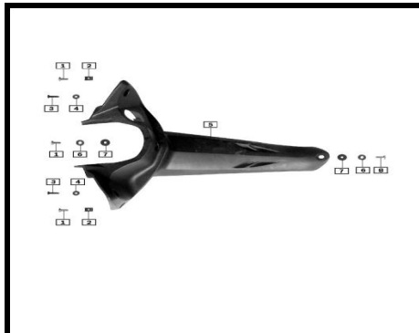
F-34 CARENAGE CENTRAL
