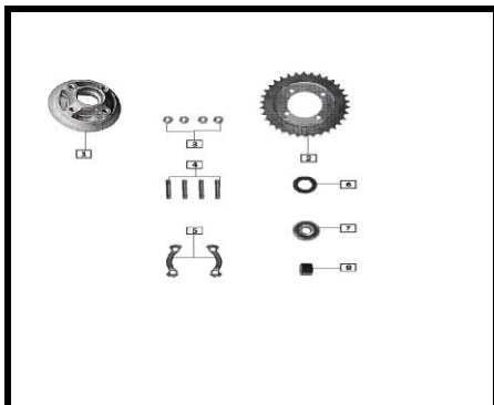
F-23 PORTA SPROCKET
