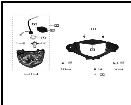
F-6 MANUBRIO
