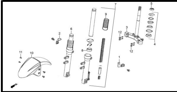
F- 9 SUSPENSION DELANTERA
