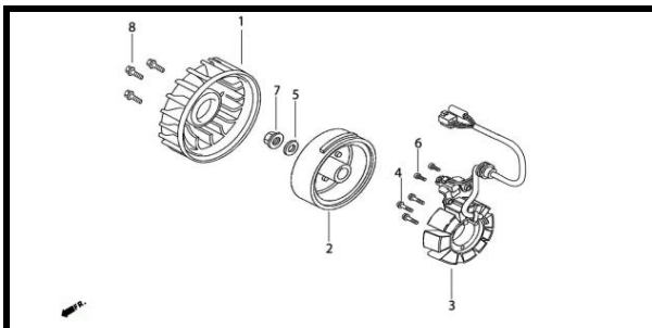
E-10 ARRANQUE ELECTRICO
